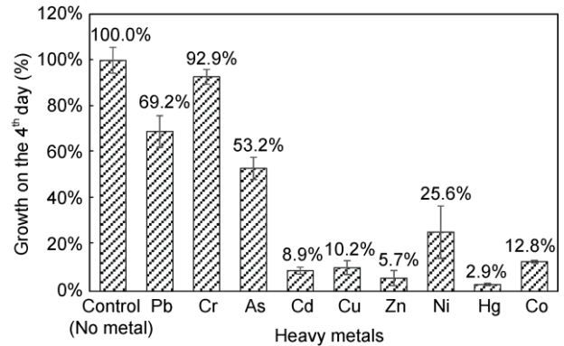
Figure 2 The growth of Rhodococcus sp. on day 4 (logarithmic phase) on 1% diesel fuel in BH media incorporated with different types of selected heavy metals ( 10 \text{ mg L}^{-1} ). The control was no-metal.
