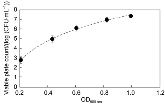
Figure 1 Standard curve for the determination of viable plate count from OD 600 nm .
