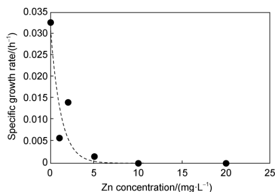
Figure 3 The specific growth rate ( \text{h}^{-1} ) at 10 \text{ }^\circ\text{C} against different concentrations of Zn. The values from the experiments are depicted as a solid markers and the model is depicted as a dashed line.
